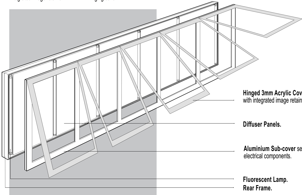
Exploded view
